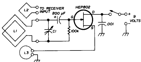
fig. 4. Loop antenna with Q-multiplier. Regeneration control is by means of L1, L3 coupling.
