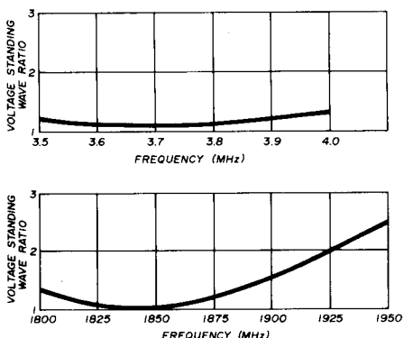
fig. 4. Vswr performance of the large vertical antenna on 80 and 160 meters.
