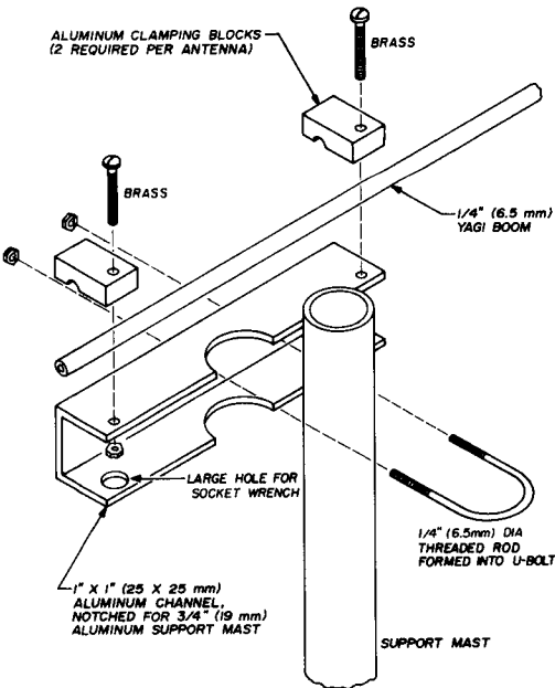
fig. 5. The Yagis are attached to the aluminum support masts with clamps (8 required) which allow all of the booms to be aligned in the same plane.
