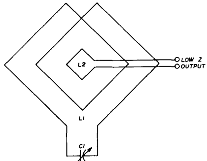
fig. 2. High- and low-impedance loop outputs.
